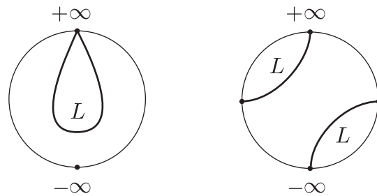
FIGURE 3: Two noncompact inessential lines.
