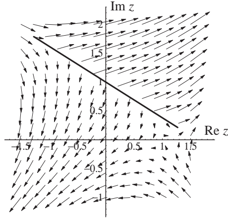
FIGURE 1. Poly plot [9] in the complex z -plane for the branch q_-(z) in the case \lambda = 1/4 - i/2 . The branch cut between the turning points at i \pm 2\sqrt{\lambda} is also shown, as is the point z = 1 at which q_-(z) vanishes.
