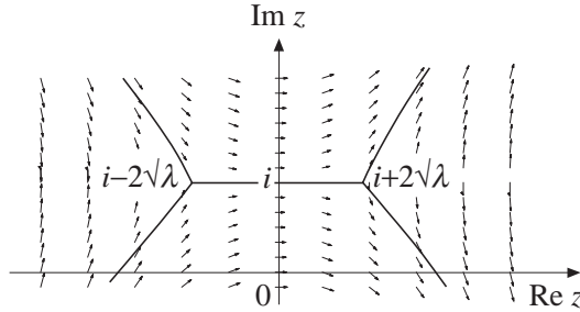
FIGURE 2. Stokes lines in the complex z -plane emanating from the turning points at i \pm 2\sqrt{\lambda} for the differential equation in the transformed form, (3) in the case of real \lambda . Note that the real axis cuts two of these lines.
